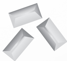
Struvietkristallen
